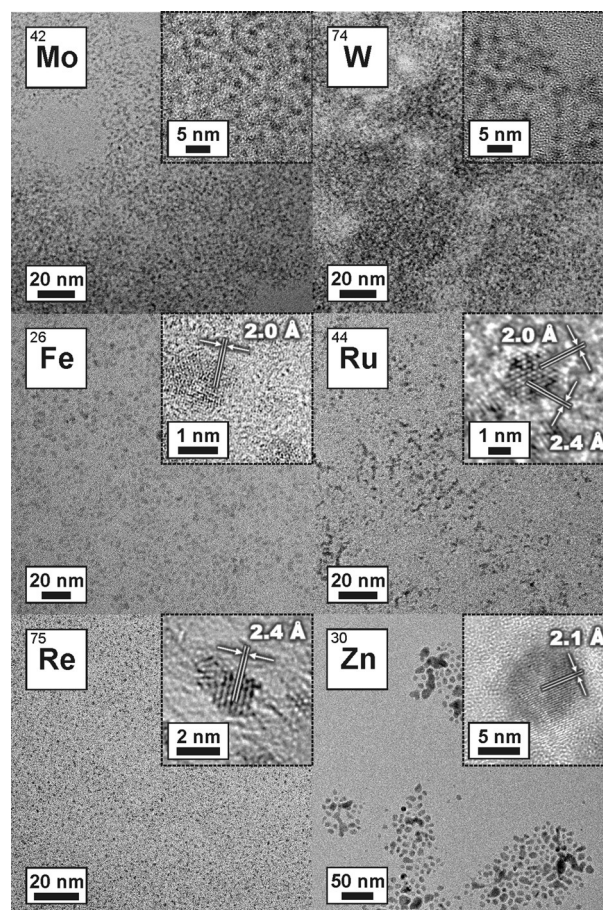
Figure 2. TEM overview and detail images (inset) of the as-prepared \text{Mo}^0 , \text{W}^0 , \text{Fe}^0 , \text{Ru}^0 , \text{Re}^0 , and \text{Zn}^0 nanoparticles (see Supporting Information for DLS, STEM, FT-IR, XRD).
