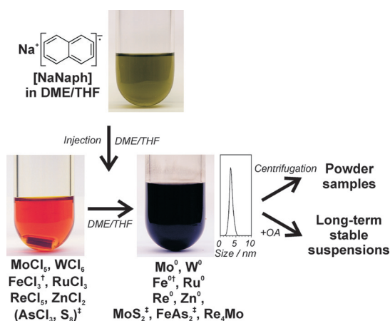
Figure 1. Scheme illustrating the synthesis of \text{Mo}^0 , \text{W}^0 , \text{Fe}^0 , \text{Ru}^0 , \text{Re}^0 and \text{Zn}^0 nanoparticles by reduction of metal chlorides with sodium naphthalenide ([NaNaph]) in ether (1,2-dimethoxyethane (DME) or tetrahydrofuran (THF)) as well as follow-up reactions to obtain \text{MoS}_2 , \text{FeAs}_2 , and \text{Re}_4\text{Mo} nanoparticles ( ^{\dagger} Photos and size distribution for the reduction of \text{FeCl}_3 to \text{Fe}^0 nanoparticles; ^{\ast} Addition of \text{S}_8 and \text{AsCl}_3 to obtain \text{MoS}_2 and \text{FeAs}_2 ; OA: oleylamine; see Experimental Section for details).
